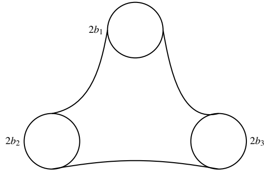
Fig. 1 A pair of pants with geodesic boundary curves of lengths 2b_1, 2b_2, 2b_3
