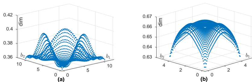
Fig. 3 (a) The plot of dimension when b is large ( b = 11 ); (b) The plot of dimension when b is smaller ( b = 4.5 ). Observe the scale.
