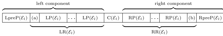
Fig. 4. Detailed structure of the 1-block \mathcal{E}_l : (a), (b) — the incomplete occurrences of periods.
